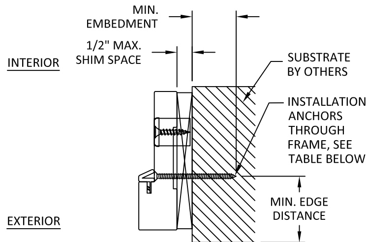
B 8 HORIZONTAL SECTION LOCK JAMB - BUTT HINGE FRAME
