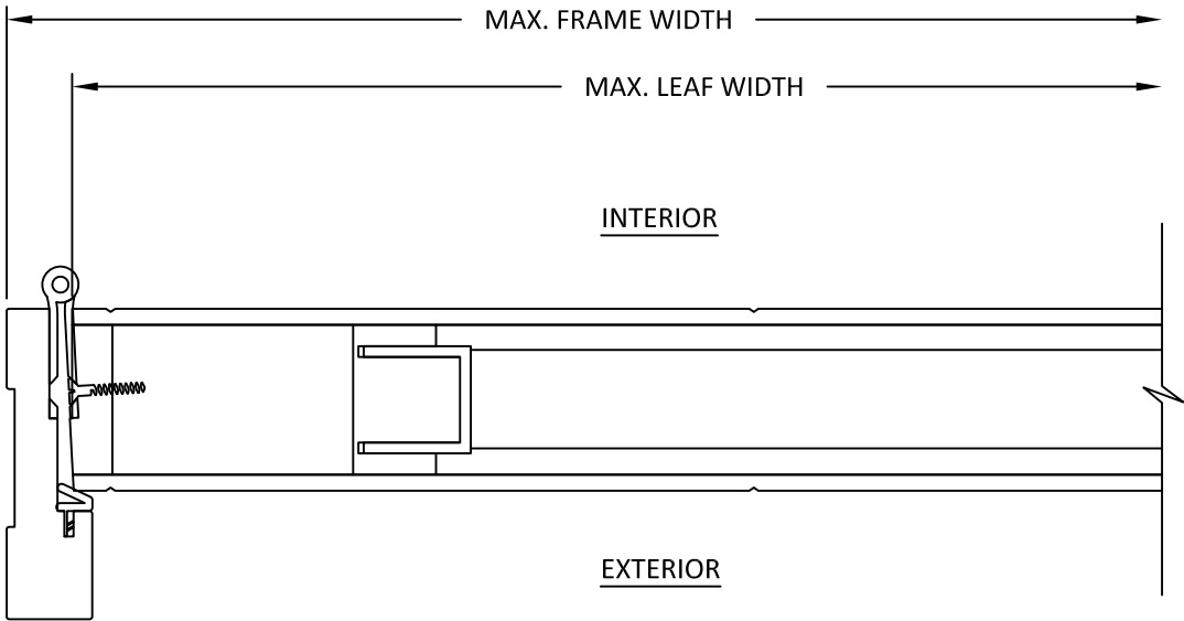
A 6 HORIZONTAL SECTION HINGE JAMB - BUTT HINGE FRAME FLUSH
