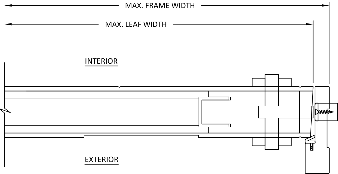
B 6 HORIZONTAL SECTION LOCK JAMB - BUTT HINGE FRAME FLUSH
