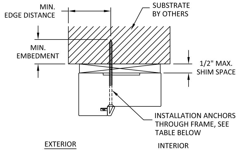
F 8 VERTICAL SECTION HEAD - CONCEALED HINGE FRAME
