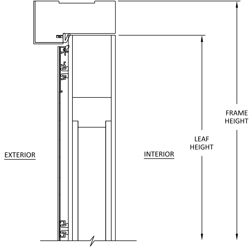
B 5 VERTICAL SECTION HEAD - CONCEALED HINGE FRAME ALUMINUM CLAD
