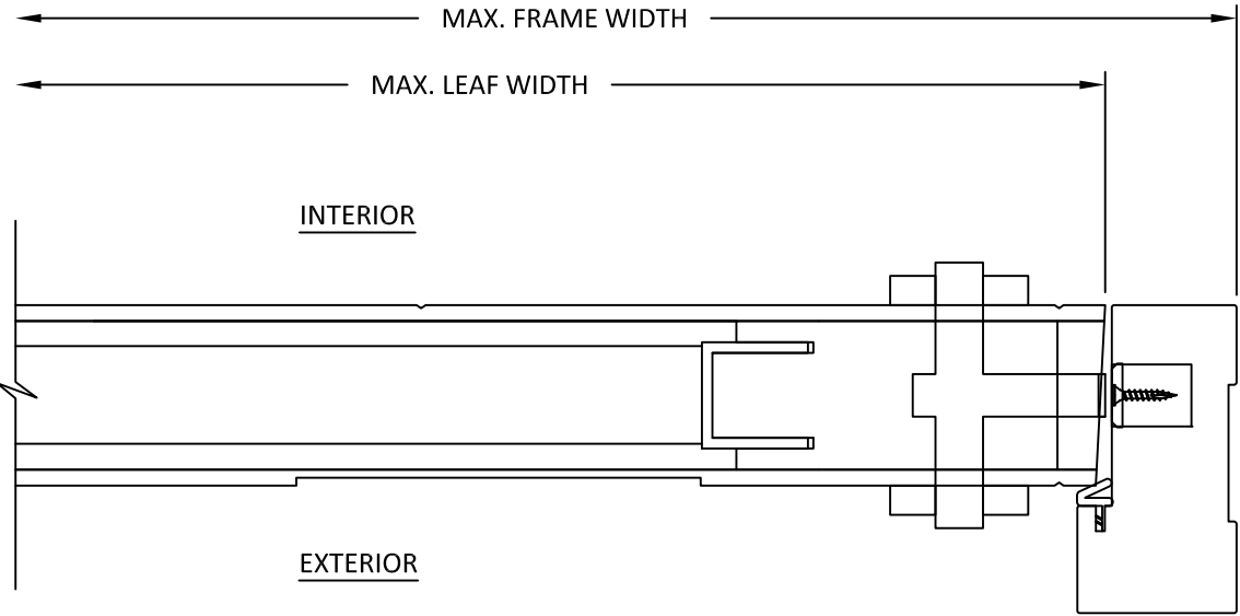
D 6 HORIZONTAL SECTION LOCK JAMB - CONCEALED HINGE FRAME FLUSH
