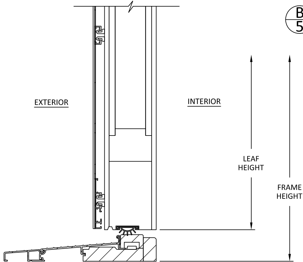
C 5 VERTICAL SECTION SILL ALUMINUM CLAD
