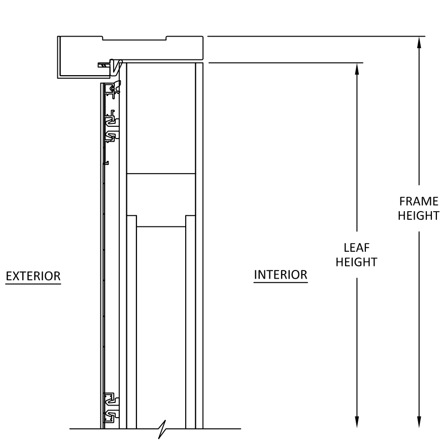
A 5 VERTICAL SECTION HEAD - BUTT HINGE FRAME ALUMINUM CLAD
