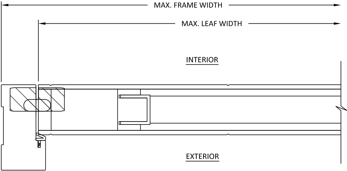
C 6 HORIZONTAL SECTION HINGE JAMB - CONCEALED HINGE FRAME FLUSH
