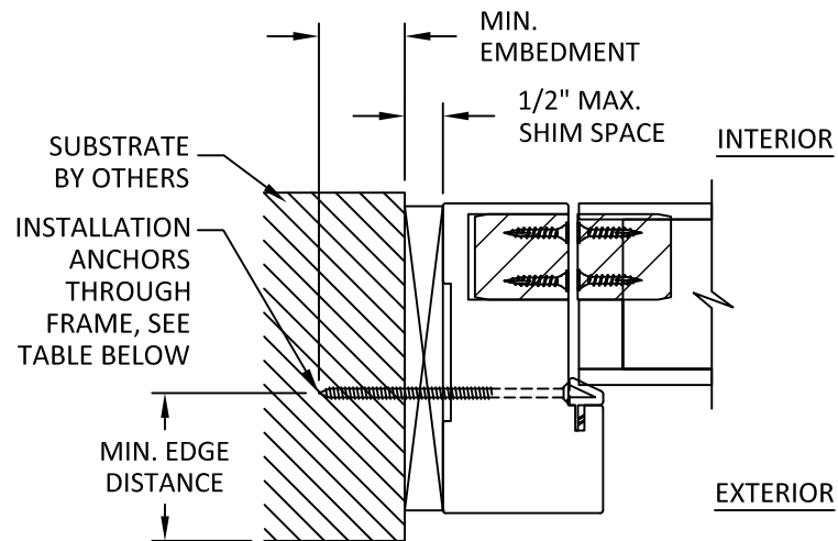
A 8 HORIZONTAL SECTION HINGE JAMB - BUTT HINGE FRAME
