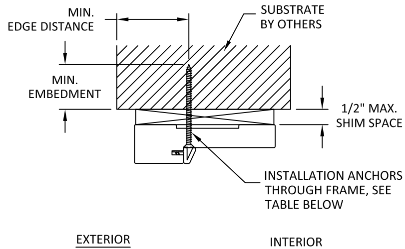
C 8 VERTICAL SECTION HEAD - BUTT HINGE FRAME
