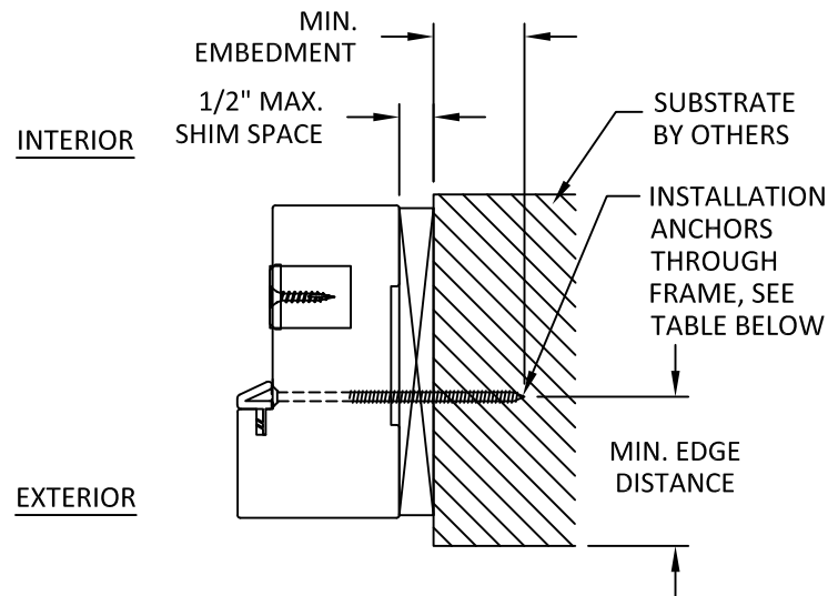
E 8 HORIZONTAL SECTION LOCK JAMB - CONCEALED HINGE FRAME
