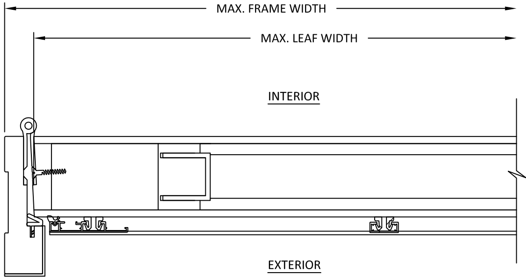
A 7 HORIZONTAL SECTION HINGE JAMB - BUTT HINGE FRAME ALUMINUM CLAD
