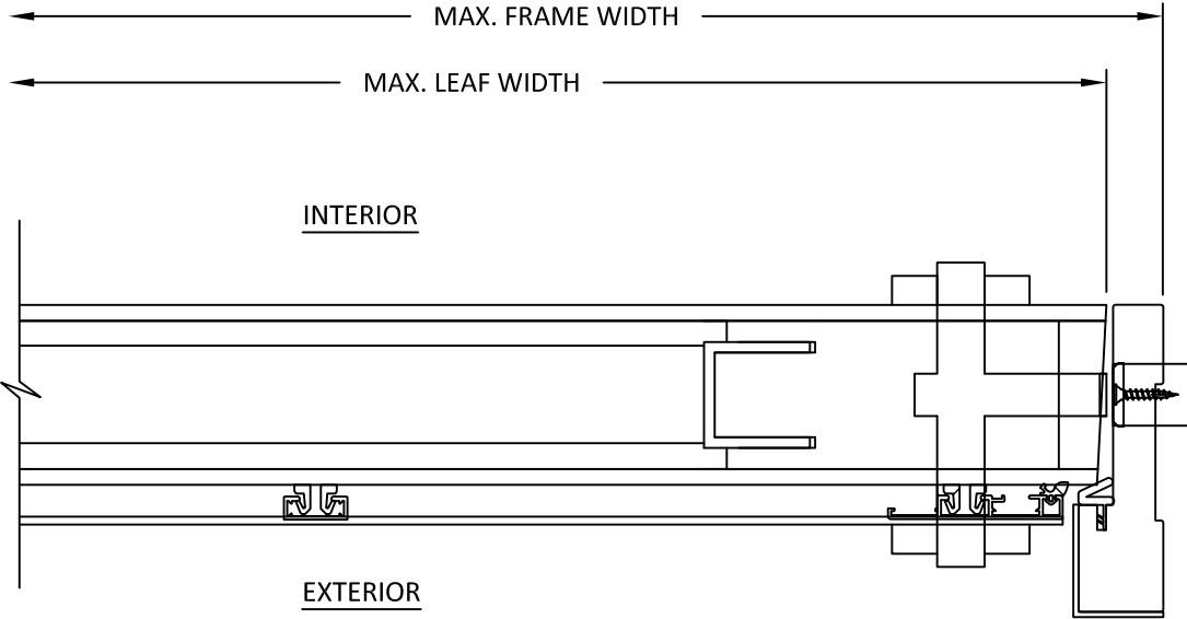
B 7 HORIZONTAL SECTION LOCK JAMB - BUTT HINGE FRAME ALUMINUM CLAD
