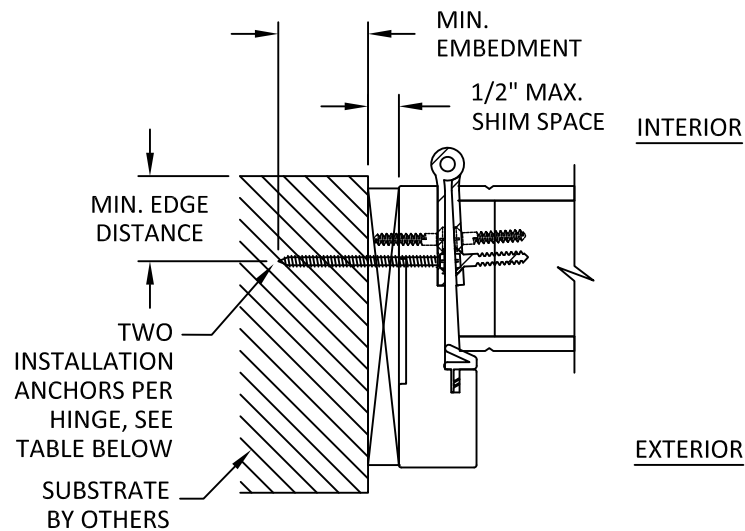
A 8 HORIZONTAL SECTION HINGE JAMB - BUTT HINGE FRAME
