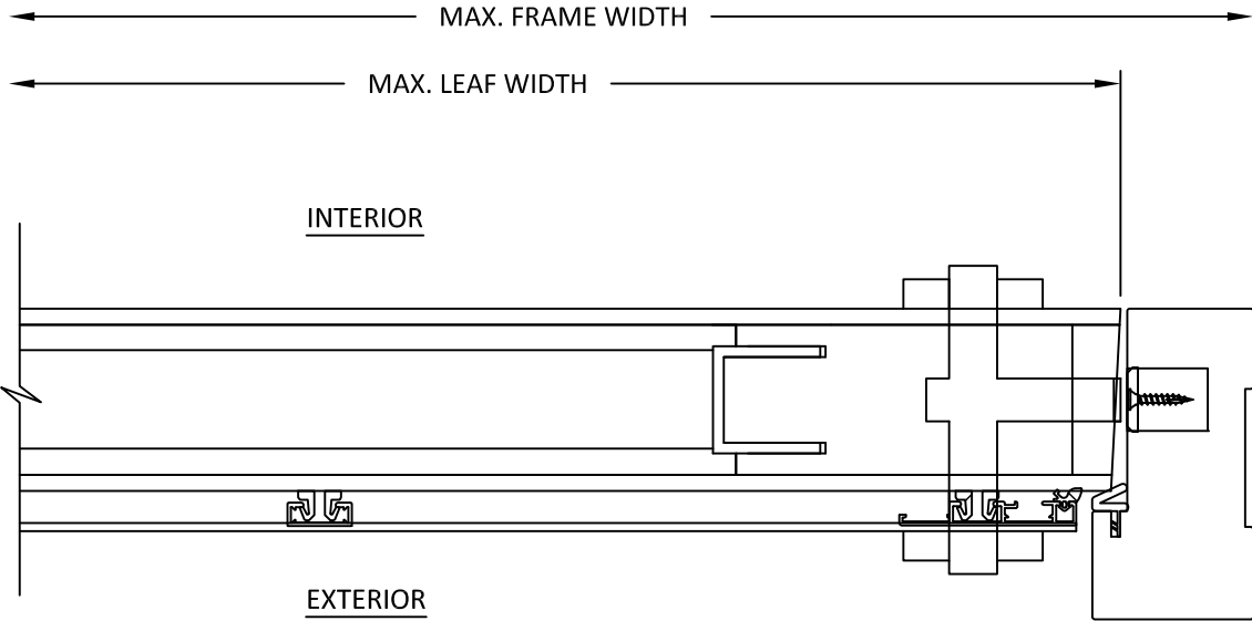
D 7 HORIZONTAL SECTION LOCK JAMB - CONCEALED HINGE FRAME ALUMINUM CLAD
