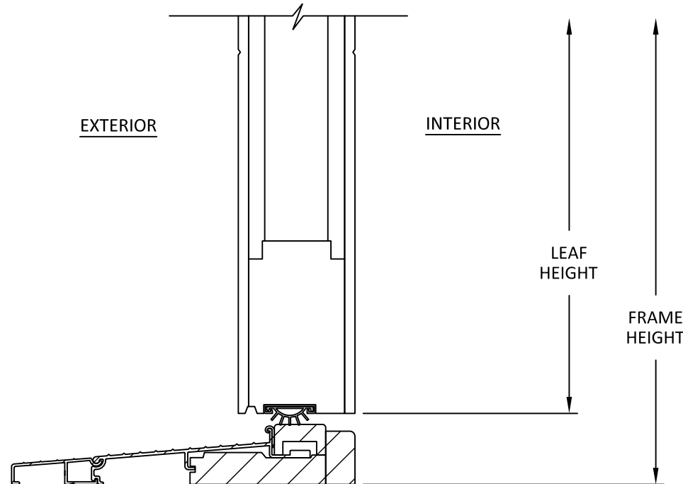
C 4 VERTICAL SECTION SILL FLUSH
