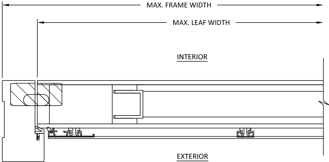
C 7 HORIZONTAL SECTION HINGE JAMB - CONCEALED HINGE FRAME ALUMINUM CLAD
